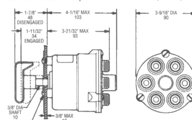
Models 72-R mounting dimensions 7/32" (6 mm) mtg holes for three 10-32 screws spaced at 120° on 1-1/4" (32 mm) radius
