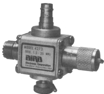
MODEL 4273-030
