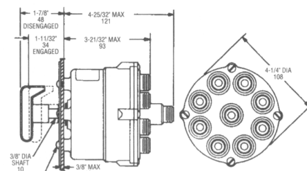
Models 74/72-2 mounting dimensions 7/32" (6 mm) mtg holes for four 10-32 screws spaced at 90° on 1-5/16" (33 mm) radius
