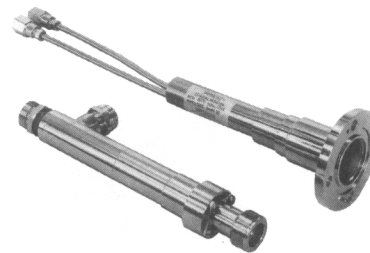
MODEL 8720 (TOP)
