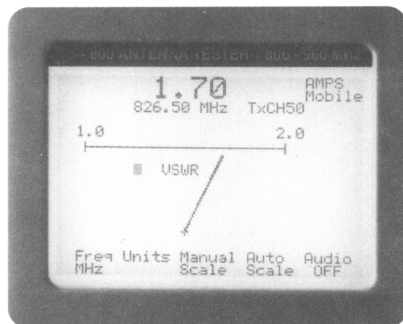
Single frequency mode for antenna tuning.
