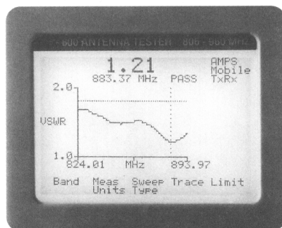
Swept frequency mode reveals a comprehensive pic- ture of antenna matching.
